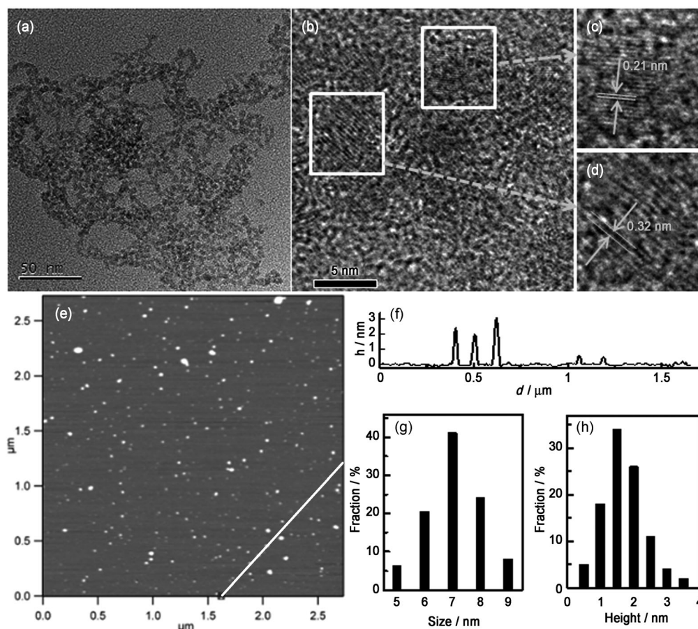
Figure 1. a) TEM and b) HRTEM images of the N,S-CDs. c),d) Typical single CDs with lattice parameters of 0.21 nm and 0.32 nm, respectively. e) AFM image of the N,S-CDs. f) Height profile along the line in (e). g),h) Size and height distributions of the N,S-CDs.
