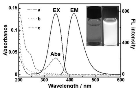
Figure 3. FL spectra (solid lines) of the obtained N,S-CDs and UV/Vis absorption spectra (dotted lines) of CA (a), L-cysteine (b), and the obtained N,S-CDs (c). Inset: Photograph of the obtained N,S-CDs under illumination of white light (left) and UV (365 nm) light (right).
